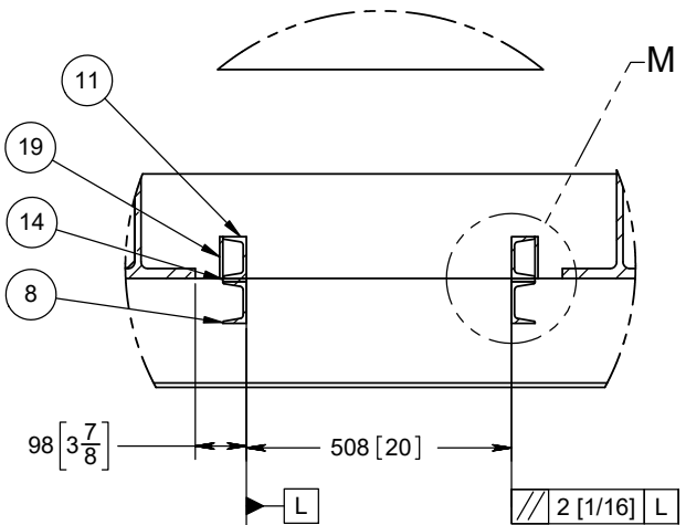
DETAIL L
