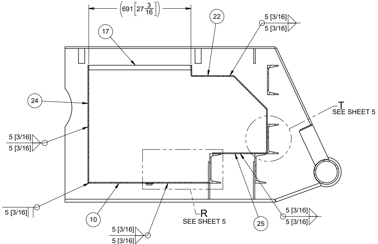
SECTION H-H
