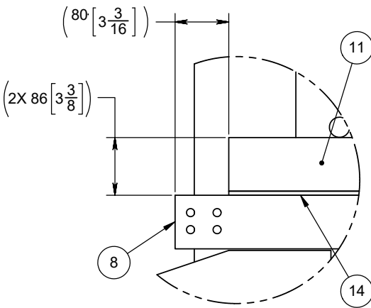
DETAIL K SCALE 1 : 4
