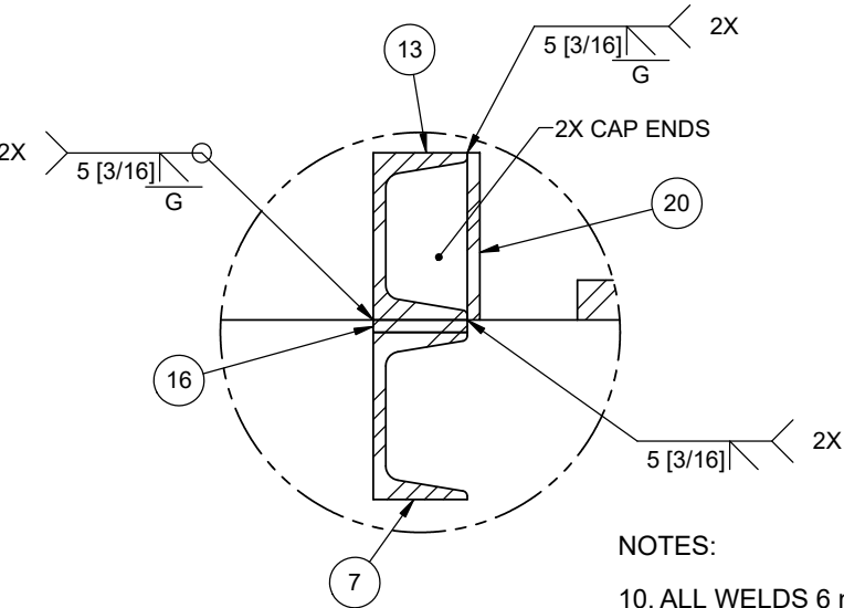
DETAIL M SCALE 1 : 2
