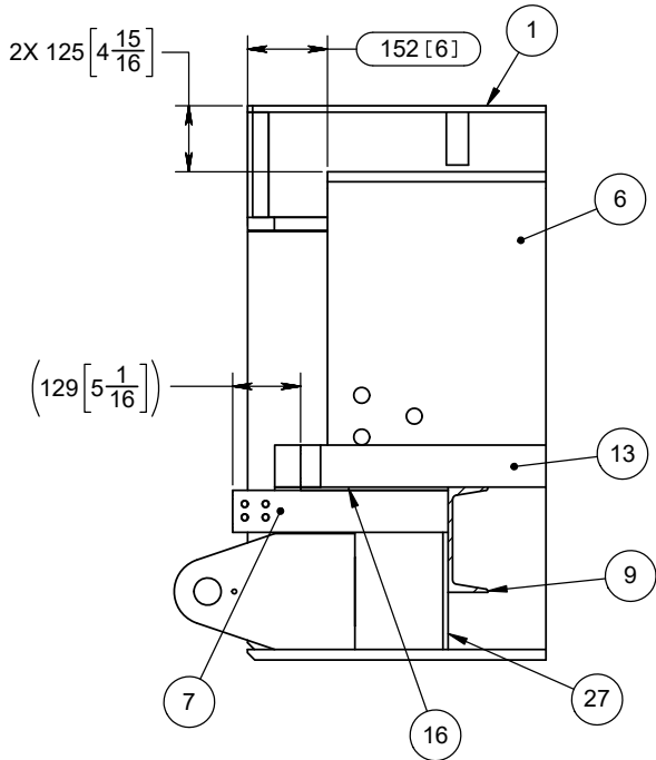
SECTION G-G
